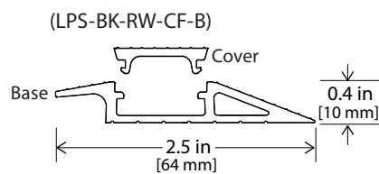
LPS Raceway Carpet to Floor (LPS-BK-RW-CF-B)
