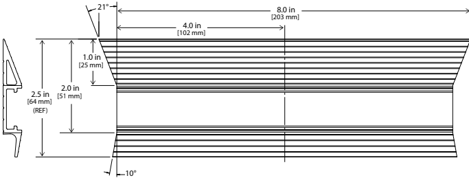
Raceway Riser (LPS-BK-RW-RSR)
