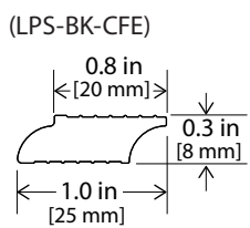
LPS Carpet Flap Extension (LPS-BK-CFE)
