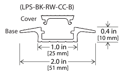
LPS Raceway Carpet to Carpet (LPS-BK-RW-CC-B)
