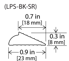
LPS Step Reducer (LPS-BK-SR)
