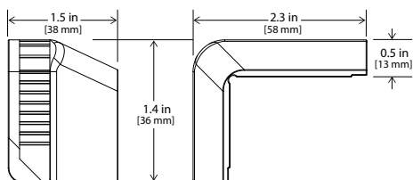
LPS Step Nose End Cap for use with Carpet Edge (LPS-BK-EC2-L/R)
