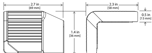
LPS Step Nose End Cap for use with Raceway (LPS-BK-EC-L/R or LPS-GY-EC-L/R)
